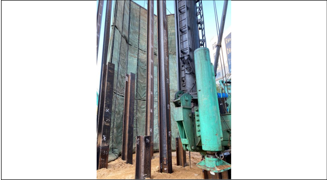
Hoisting of noise barrier during piling
